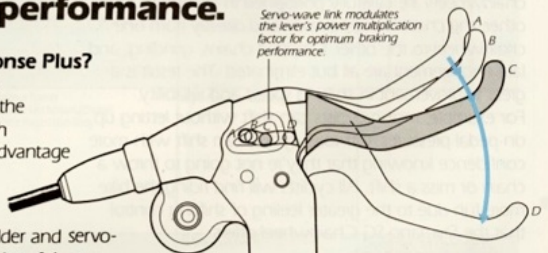
A-B stroke brings shoes quickly into contact with rim. B-C stroke slows cable take-up. C-D stroke increases power multiplication factor for super-strong but easily modulated braking power.
