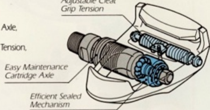
Cartridge Axle Easy-Maintenance
