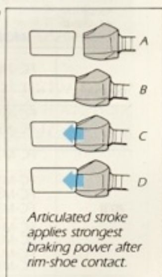
A-B stroke brings shoes quickly into contact with rim. B-C stroke slows cable take-up. C-D stroke increases power multiplication factor for super-strong but easily modulated braking power.
